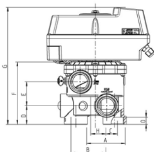
Side Mount
