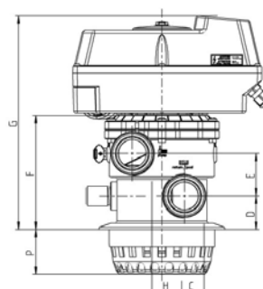
Top Mount *
